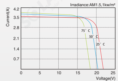
SLP050-12U I-V Curves
