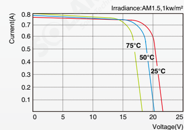
SLP012-12 I-V Curves
