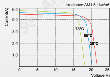
SLP090-12C1D2 I-V Curves
