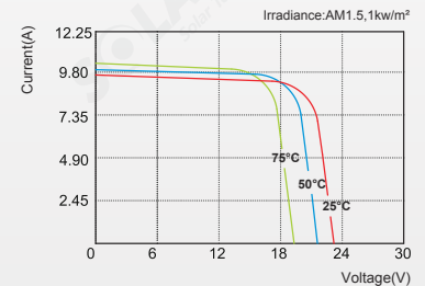
SLP175S-12 I-V Curves
